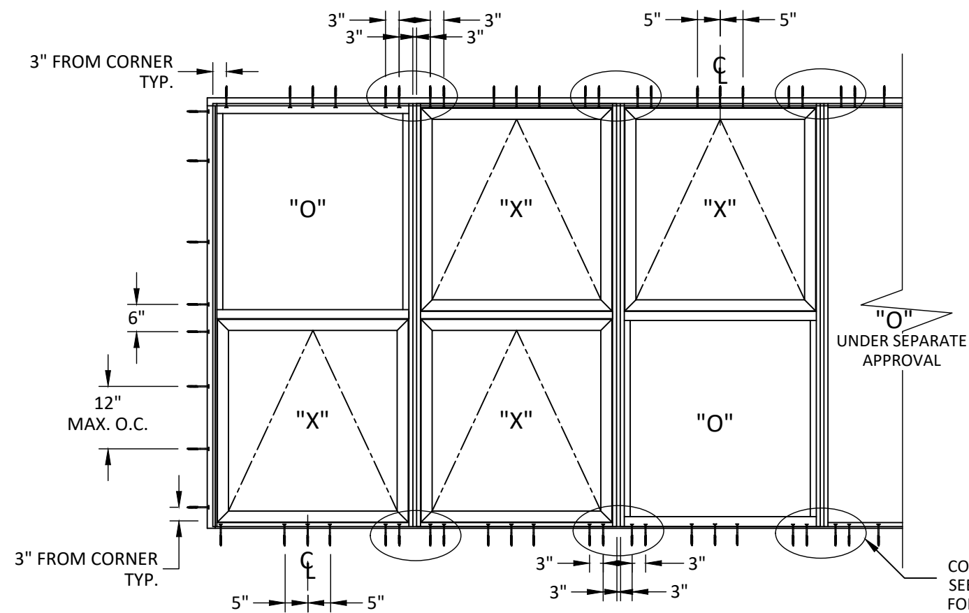
ANCHOR LAYOUT STRAP, CLIP, TRIM/CLIP, TWIST ANCHOR OR THRU FRAME INSTALLATIONS
