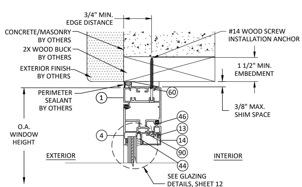
07 VERTICAL SECTION VENT HEAD - 2X WOOD BUCK THROUGH FRAME - TYP.
