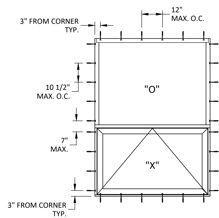
ANCHOR LAYOUT ALL INSTALLATIONS
